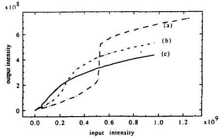
Fig. 4 Response for different values of the thickness: (a) D=5\mu\text{m} ; (b) D=5.026\mu\text{m} ; (c) D=5.043\mu\text{m} . \alpha=2000\text{ m}^{-1} ; n_0=3.56 ; \chi^{(3)}=10^{-12}\text{ m}^2/\text{V}^2 ; \lambda=1.06\mu\text{m}
