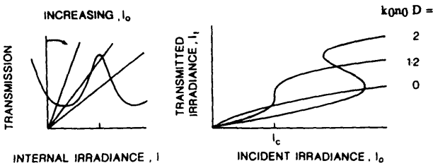
Fig.1 Graphical solution of the set of equations (2.13,15,18). From [4].
