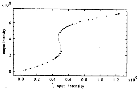
Fig. 3 Comparison between simulation results and analytical data [5]. ..... analytical results; +: simulation points. D=5\mu\text{m} , \alpha=1000\text{ m}^{-1} ; n_0=3.56 ; \chi^{(3)}=10^{-12}\text{ m}^2/\text{V}^2 ; \lambda=1.06\mu\text{m}
